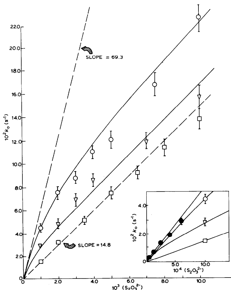
Fig. 1. Variation of k_0 with [\text{S}_2\text{O}_3^{2-}] at four concentrations of \text{OH}^- : [\text{OH}^-] = 9.87 \times 10^{-2} \text{ M} ( \bullet ); 6.16 \times 10^{-2} \text{ M} ( \circ ); 1.38 \times 10^{-2} \text{ M} ( \nabla ); and 3.16 \times 10^{-4} \text{ M} ( \square ); T = 25.0^\circ\text{C} , ionic strength, 0.10M.
